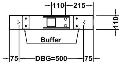
Pillar 60x60x3 H MAX=3500 mm
