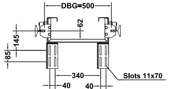
Upper Cabin Fastening
